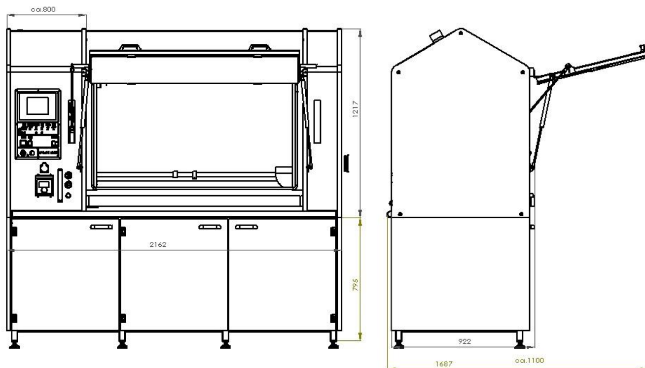
Figure 3 Mechanical dimensions CCT 1000-FL-I
