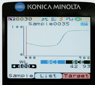
Spectral graph
